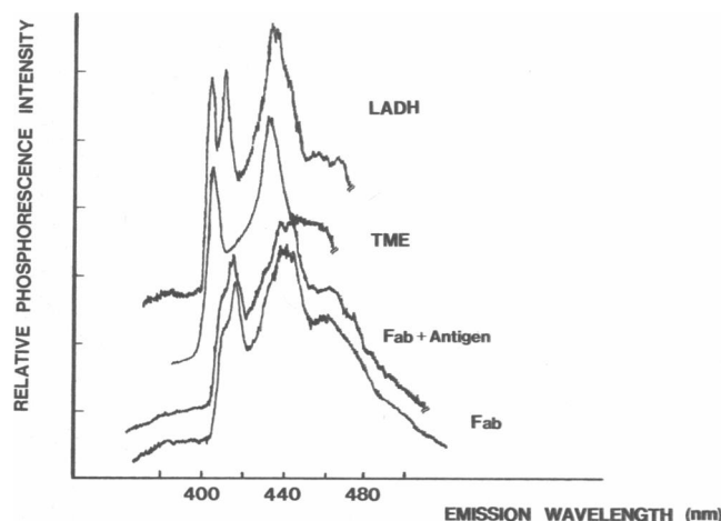
FIGURE 1 The phosphorescence spectra of the Fab' fragment of IgA J539 ( 1.5 \times 10^{-5} M) in the presence and absence of the gal 4 antigen ( 1.0 \times 10^{-4} M) using 2:1 glycerol/phosphate buffer (pH 7.4) as the solvent. Tryptophan methyl ester and LADH in the same solvent are shown for comparison. The spectra were all obtained at 77 K, and are displayed with excitation at 280 nm.
